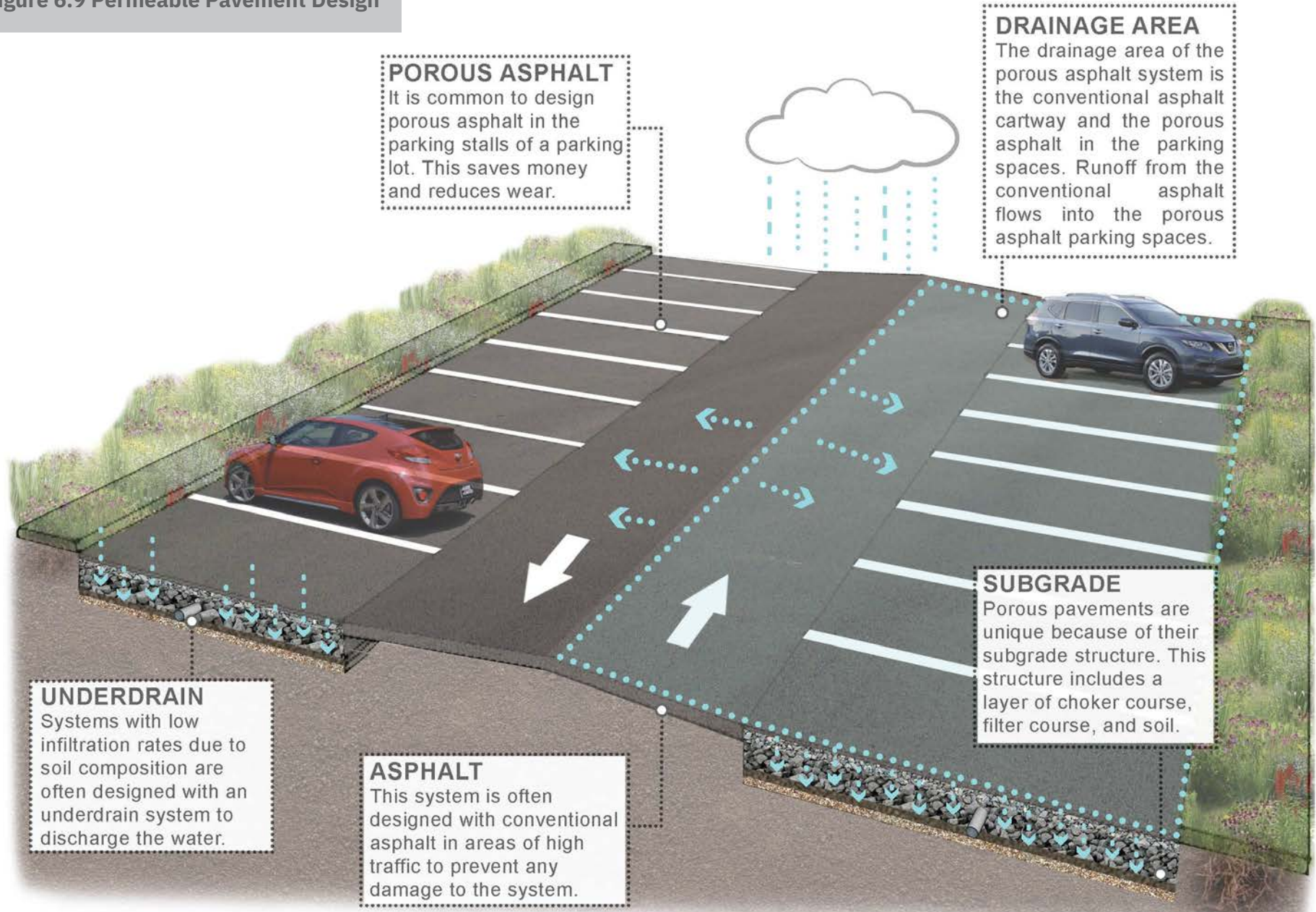
Figure 6.9 Permeable Pavement Design
